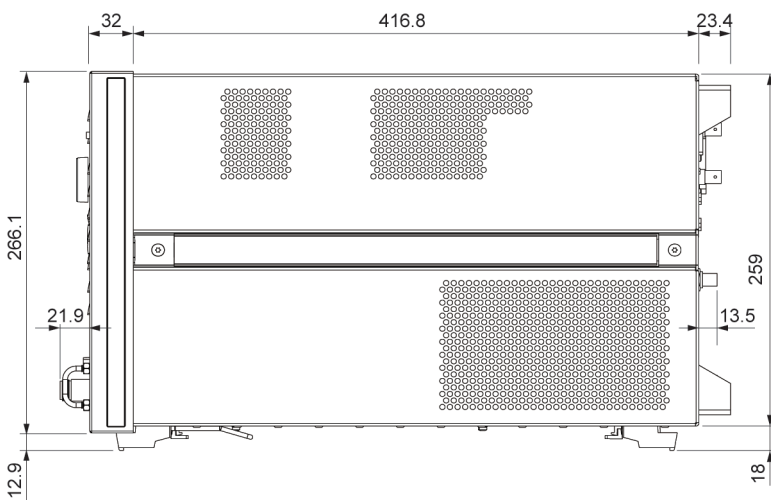
Figure 8-3. Side view
